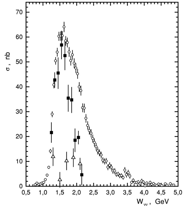
FIG. 1. The L3 preliminary data on the \gamma\gamma \rightarrow \pi^+\pi^-\pi^+\pi^- cross section [8] (open circles) and the ARGUS data on the (J^P, |J_z|) = (2^+, 2) partial cross section for \gamma\gamma \rightarrow \rho^0\rho^0 [10] (full squares) and \gamma\gamma \rightarrow \rho^+\rho^- [11] (open triangles).
